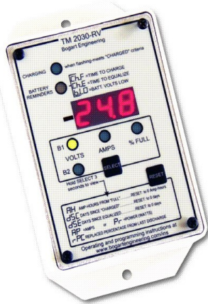
TM-2030-RV details
