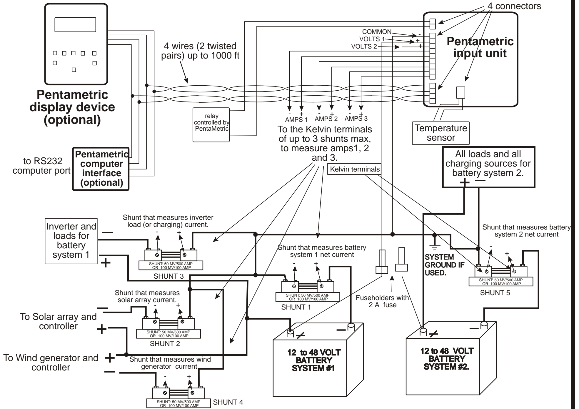
FIGURE 1: PENTAMETRIC TYPICAL BATTERY MONITOR CONNECTIONS.
